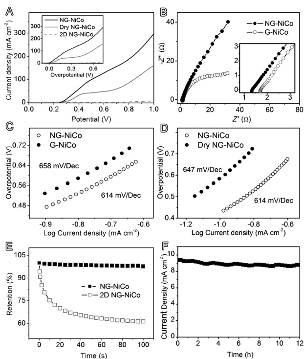
Figure 3. A) LSV plots of NG-NiCo, dried NG-NiCo, and 2D NG-NiCo at 50 mV s -1 in 0.1 M KOH; the inset in (A) shows the corresponding data re-plotted as the current density vs. overpotential. B) EIS spectra of NG-NiCo and G-NiCo. C), D) Tafel plots for NG-NiCo in comparison to those for G-NiCo and dried NG-NiCo. E) Retention percentage of the catalytic current for NG-NiCo and 2D NG-NiCo (0.7 V vs. Ag/AgCl) during the initial 100 s. F) Chronoamperometric response for NG-NiCo at 0.5 V vs. Ag/AgCl.
